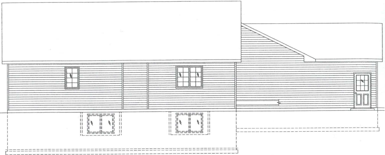
REAR ELEVATION
